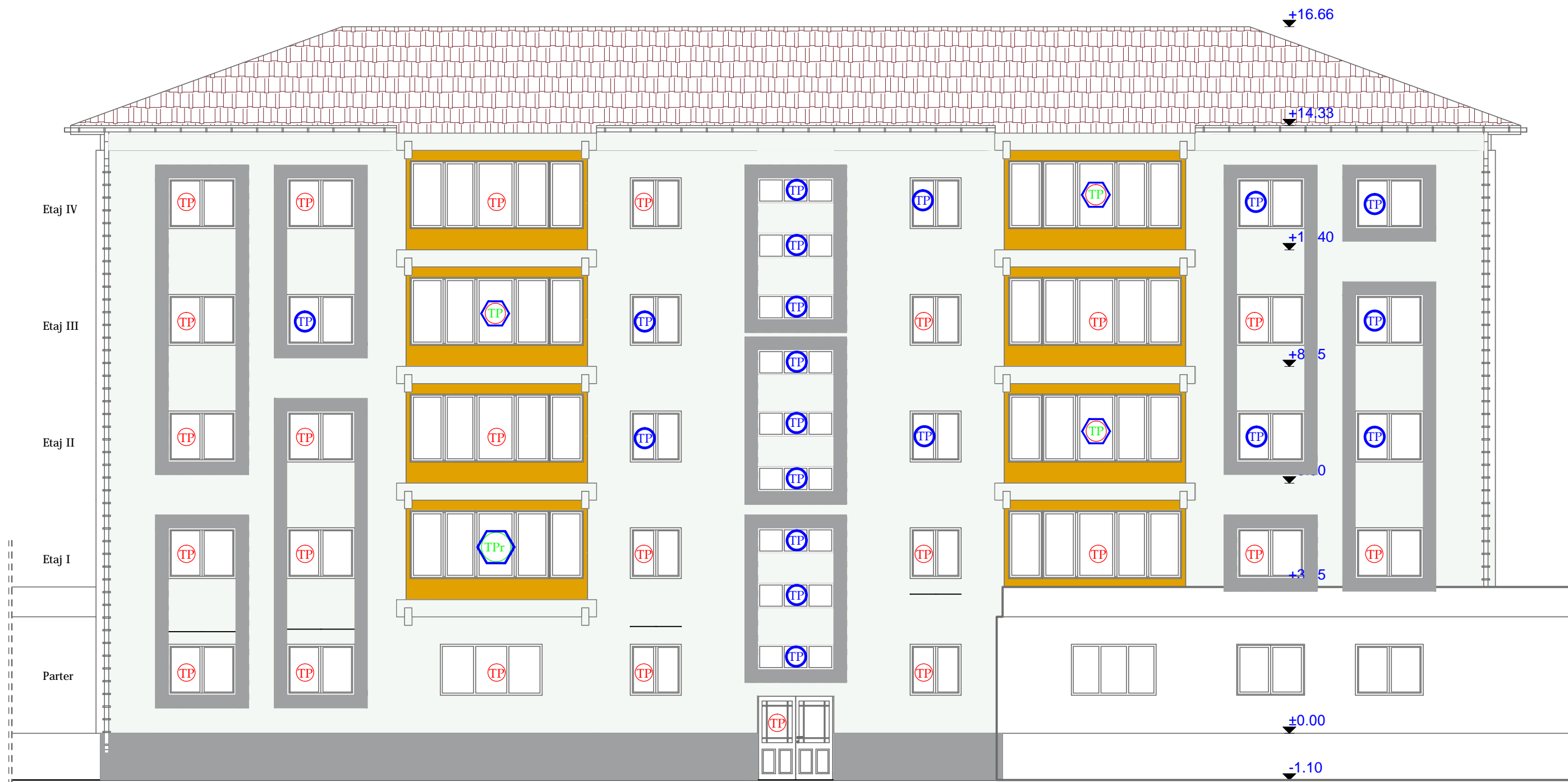
FATADA PRINCIPALA (propus)
